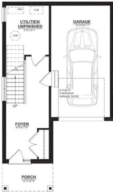
GROUND LEVEL
