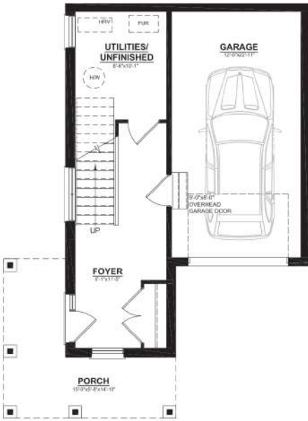
GROUND LEVEL
